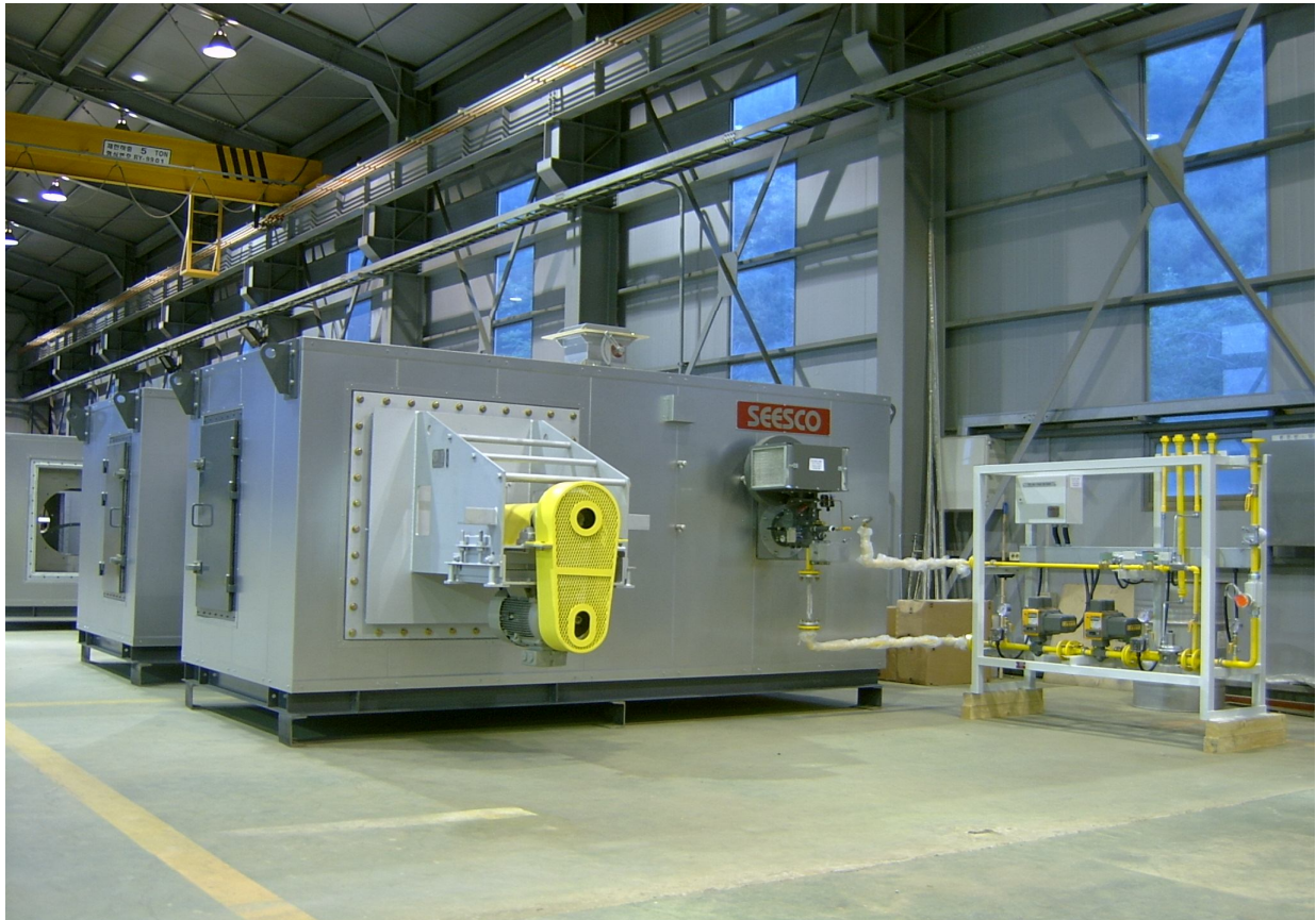
Direct fired Heater Unit for radiation oven
